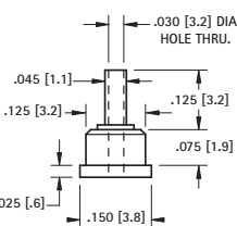
Bottom Mount
