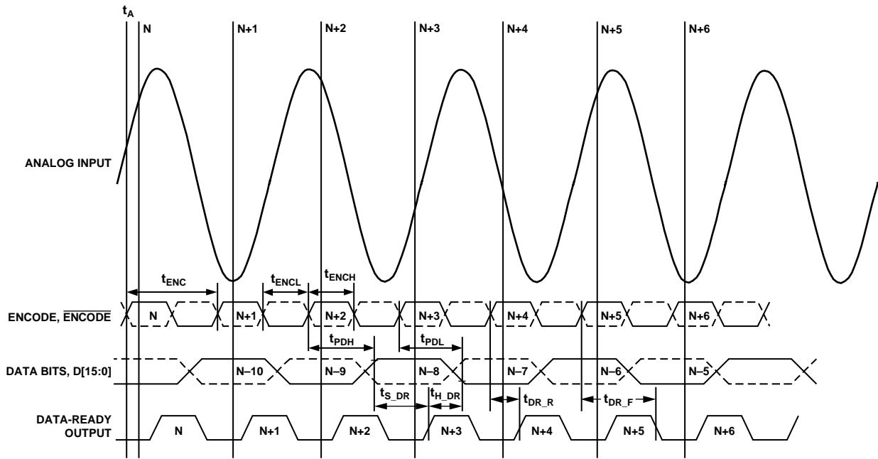
Figure 2. Timing Diagram
