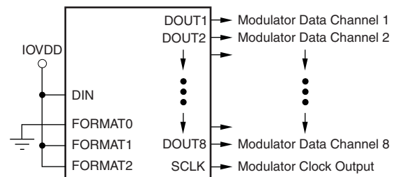
Figure 81. Modulator Output
