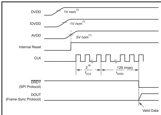
Figure 80. Start-Up Sequence
