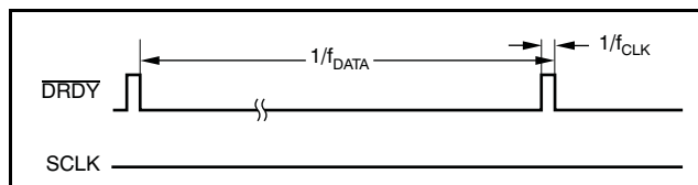
Figure 72. \overline{\text{DRDY}} Timing with No Readback
