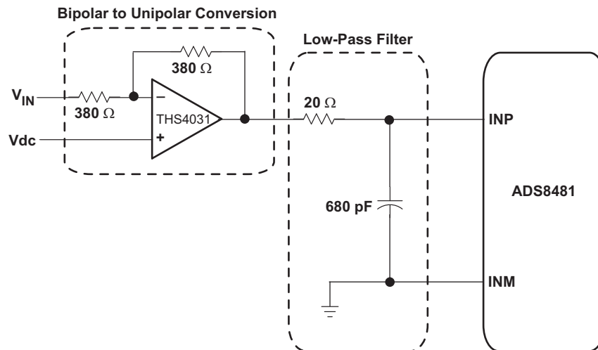
Figure 41. Input Circuit
