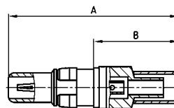
Plug contact
