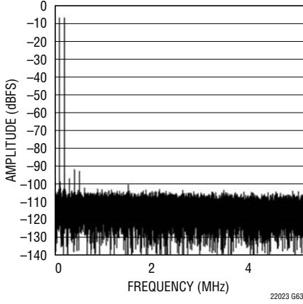
LTC2202: 32K Point 2-Tone FFT, f_{IN} = 60.2\text{MHz} and 70.1\text{MHz} , -7\text{dBFS} , \text{PGA} = 0
