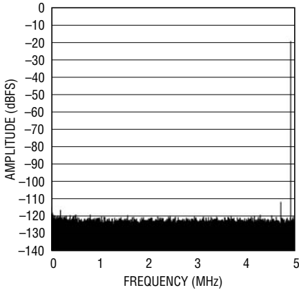
LTC2203: 128K Point FFT, f IN = 5.1MHz, -20dBFS, PGA = 0, Internal Dither "On"
