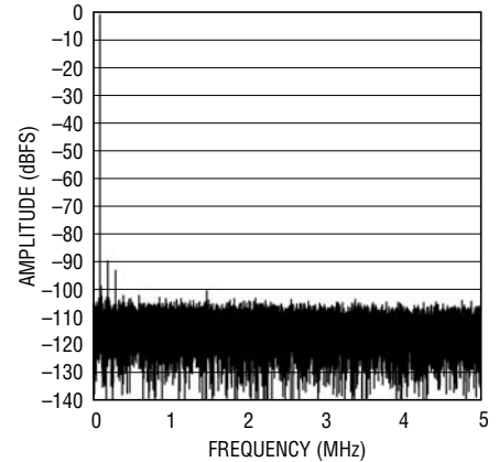
LTC2202: 32K Point FFT, f_{IN} = 70.1\text{MHz} , -1\text{dBFS} , \text{PGA} = 1
