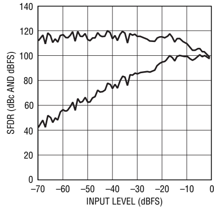
LTC2202: SFDR vs Input Level, f IN = 5MHz, PGA = 0, Dither "On"
