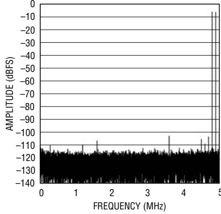
LTC2202: 32K Point 2-Tone FFT, f IN = 5.1MHz and 15.2MHz, -7dBFS, PGA = 0
