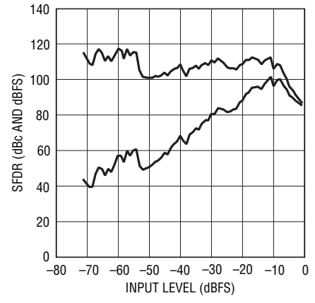
LTC2202: SFDR vs Input Level, f_{IN} = 70.1\text{MHz} , \text{PGA} = 0 , Dither "Off"
