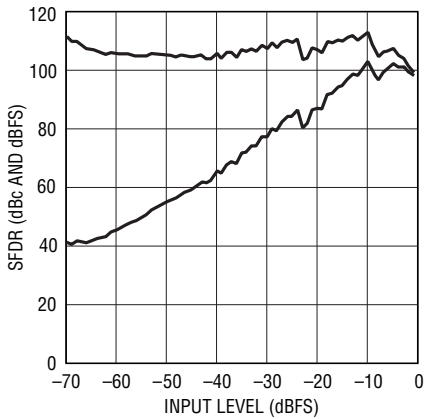
LTC2202: SFDR vs Input Level, f IN = 5MHz, PGA = 0, Dither "Off"
