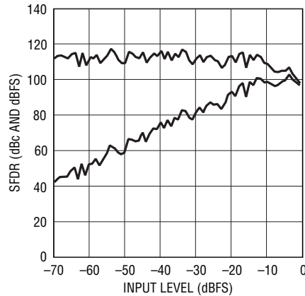
LTC2202: SFDR vs Input Level, f_{IN} = 30.1\text{MHz} , \text{PGA} = 0 , Dither "On"
