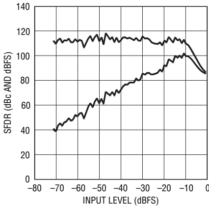
LTC2202: SFDR vs Input Level, f_{IN} = 70.1\text{MHz} , \text{PGA} = 0 , Dither "On"
