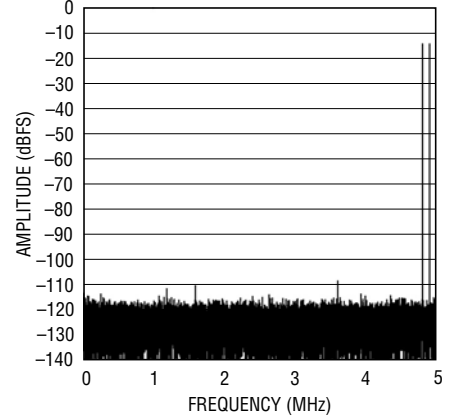
LTC2202: 32K Point 2-Tone FFT, f IN = 5.1MHz and 15.2MHz, -15dBFS, PGA = 0
