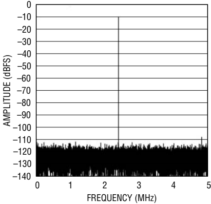
LTC2202: 32K Point FFT, f IN = 12.4MHz, -10dBFS, PGA = 0
