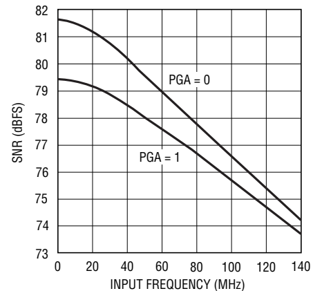
LTC2202: SNR vs Input Frequency
