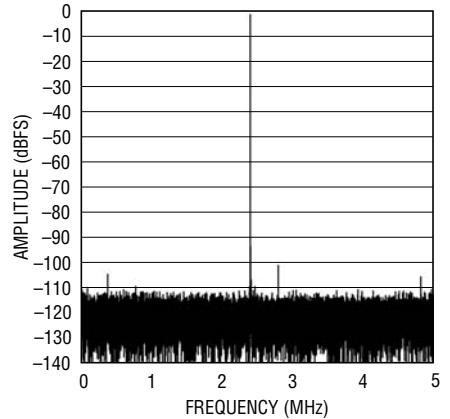
LTC2202: 32K Point FFT, f IN = 12.4MHz, -1dBFS, PGA = 0
