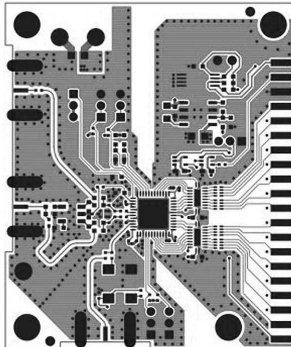
Silkscreen Topside
