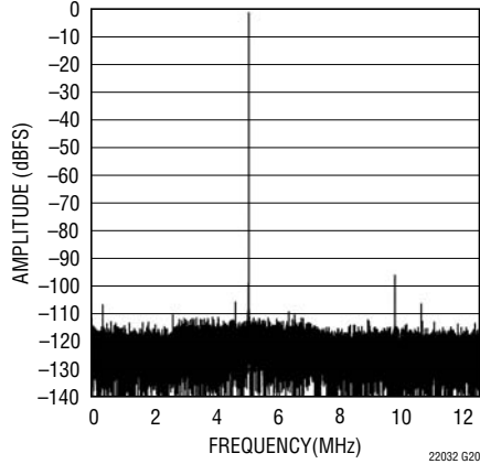
LTC2203: 32K Point FFT, f_{IN} = 30\text{MHz} , -1\text{dBFS} , \text{PGA} = 1
