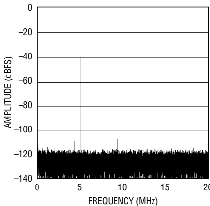
LTC2204: 64K Point FFT, 40Msps, f_{IN} = 5.1\text{MHz} , -40\text{dBFS} , \text{PGA} = 0 , \text{DITH} = 0
