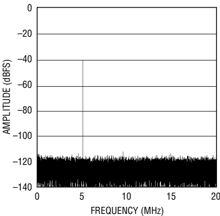
LTC2204: 64K Point FFT, 40Msps, f_{IN} = 5.1\text{MHz} , -40\text{dBFS} , \text{PGA} = 0 , \text{DITH} = 1
