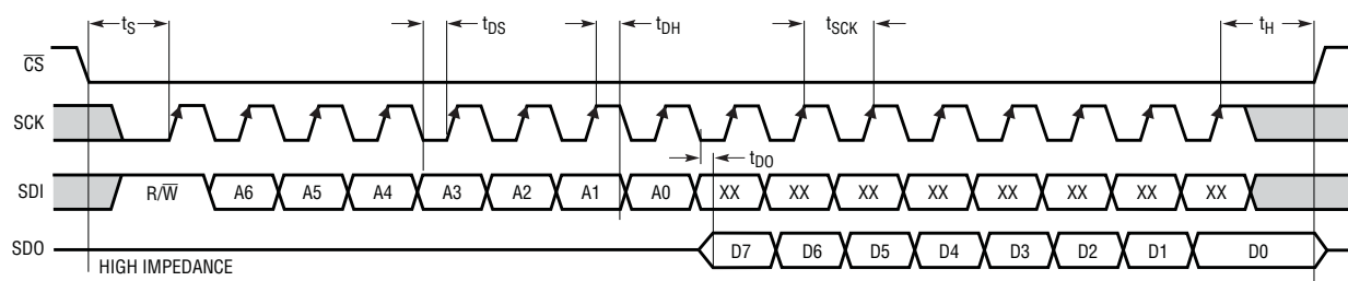
SPI Port Timing (Readback Mode)
