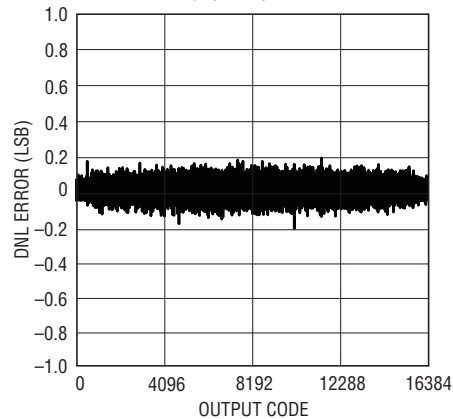
LTC2263-14: Differential Nonlinearity (DNL)
