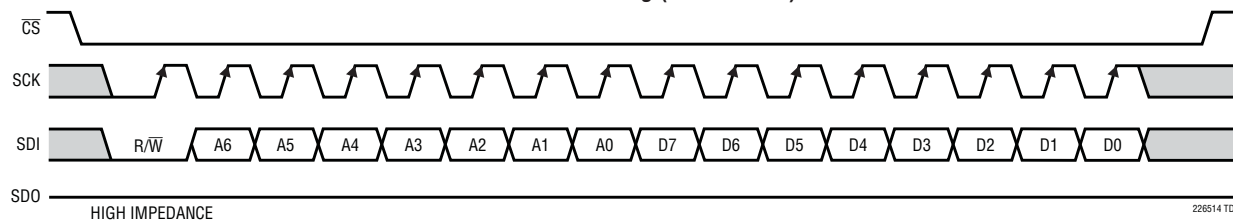
SPI Port Timing (Write Mode)
