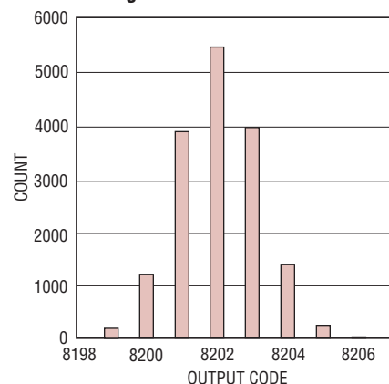
LTC2263-14: Shorted Input Histogram
