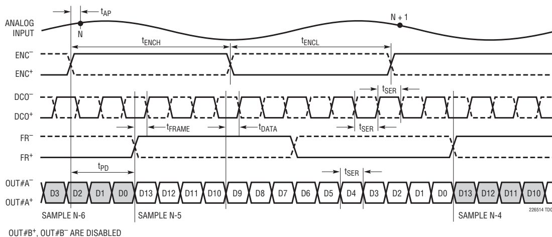
1-Lane Output Mode, 12-Bit Serialization
