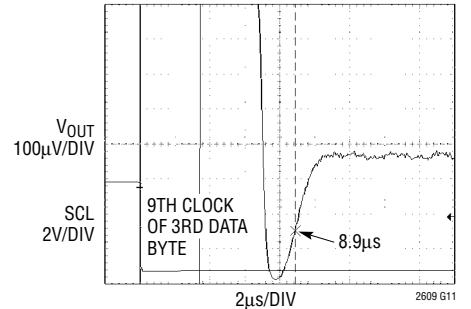
Settling to \pm 1LSB
