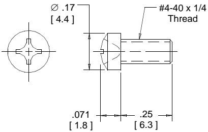
Board Lock Screw 3M Part Number 3344-4
