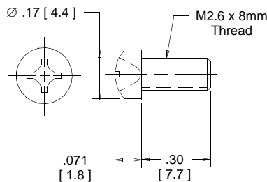
Panel Mount Screw 3M Part Number 3344-26
