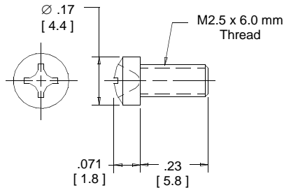
Board Lock Screw 3M Part Number 3344-3
