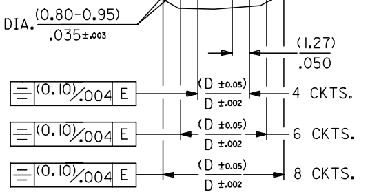
MOUNTING HOLE PATTERNS (SEE FROM COMPONENT SIDE)
