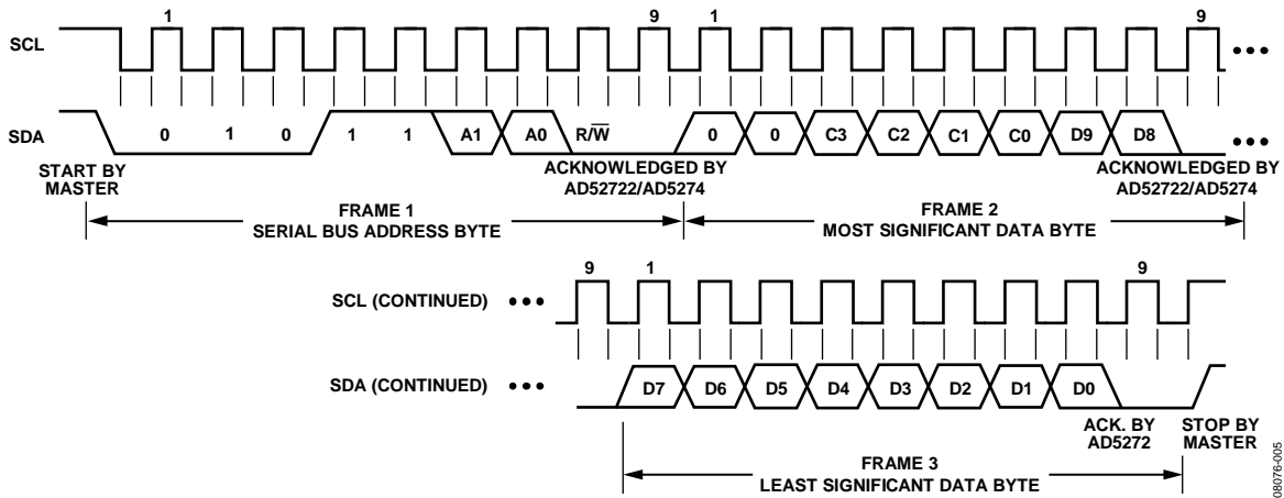
Figure 43. Write Command
