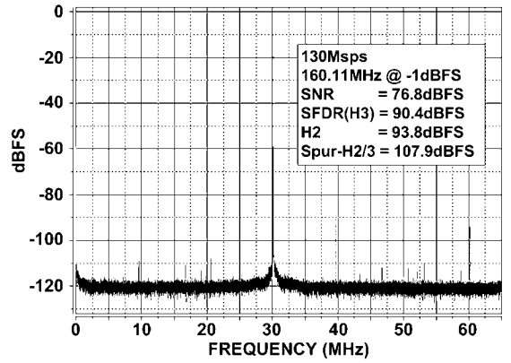
Spectral Response @ 160.11 MHz
