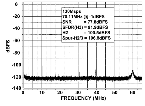
Spectral Response @ 70.11 MHz
