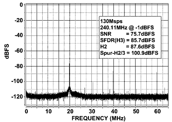
Spectral Response @ 240.11 MHz
