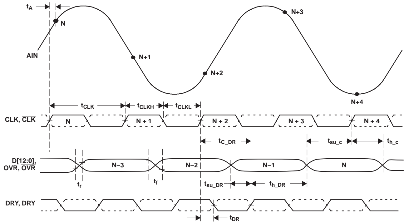
Figure 2. Timing Diagram
