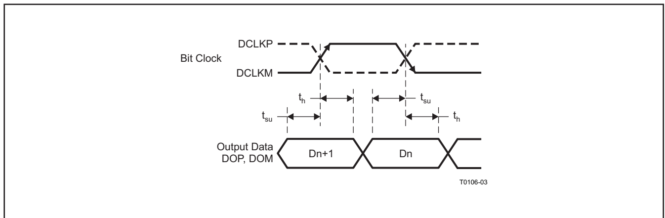
Figure 2. LVDS Timing
