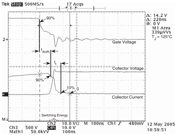
Figure 23, Turn-off Switching Waveforms and Definitions
