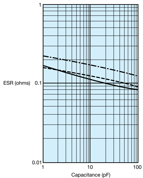
AVX CORPORATION - - - 250 MHz - - - 500 MHz — 1000 MHz
