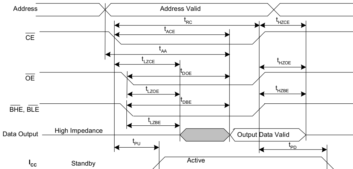
Figure 6. SRAM Read Cycle #2: \overline{CE} and \overline{OE} Controlled [3, 10, 14]
