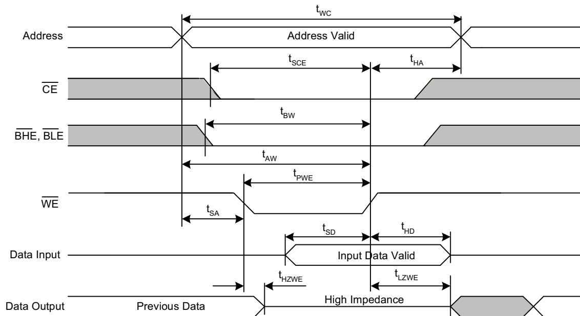
Figure 7. SRAM Write Cycle #1: \overline{WE} Controlled [3, 13, 14, 15]
