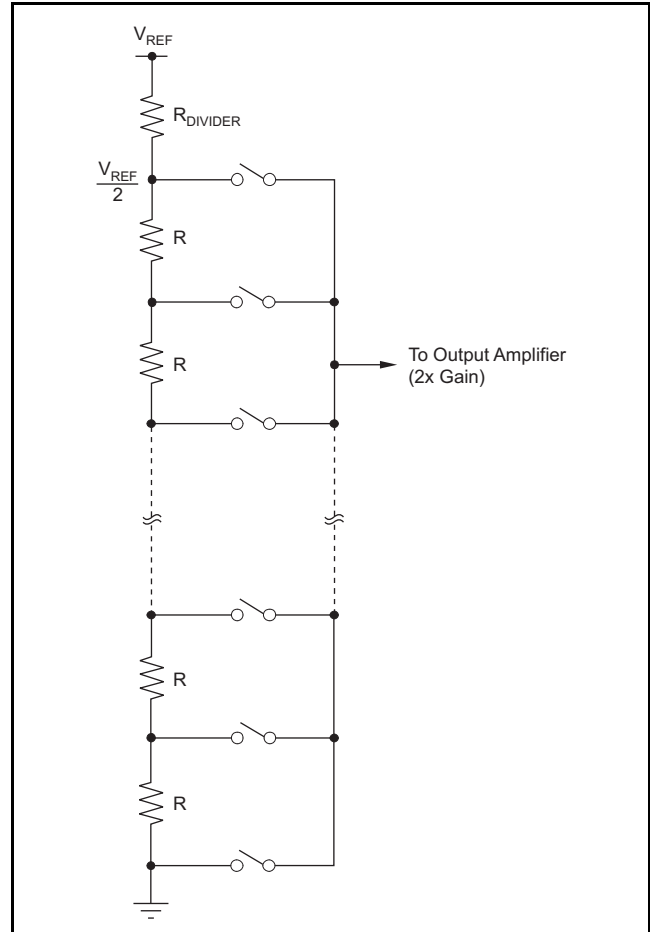
Figure 112. Resistor String
