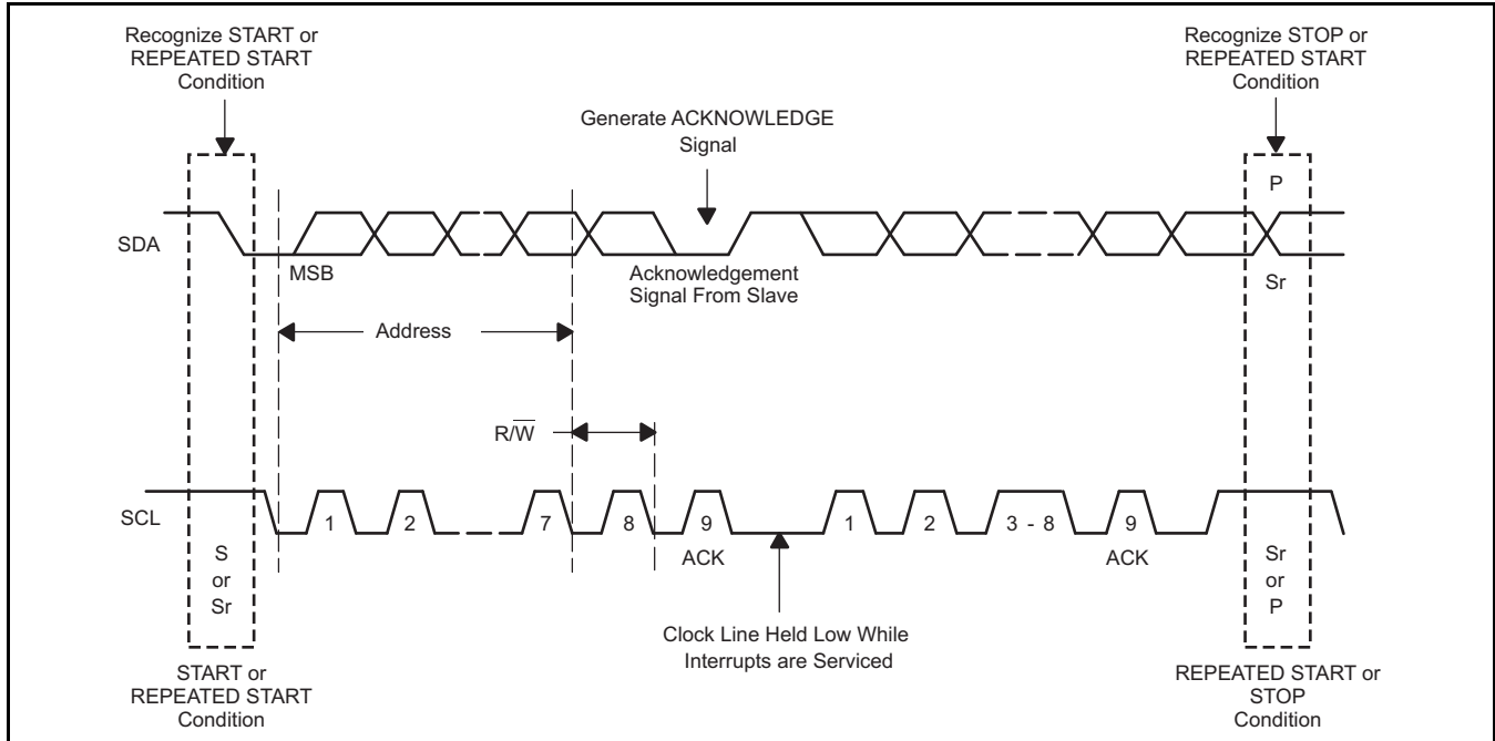
Figure 116. I 2 C Bus Protocol
