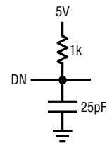
(B) V_{OL} TO Hi-Z
