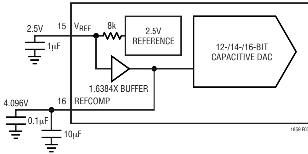
Figure 3. Internal or External Reference Source
