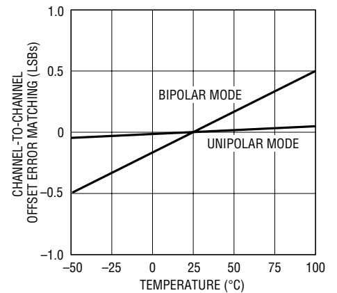
LTC1859 Channel-to-Channel Offset Error Matching vs Temperature
