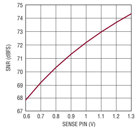
LTC2265-14: SNR vs SENSE, f_{IN} = 5\text{MHz} , -1dBFS
