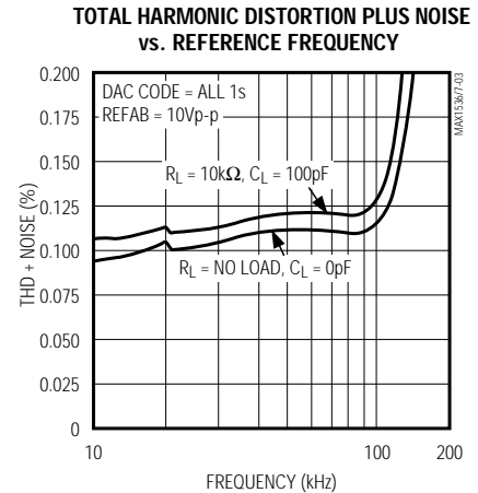
MAX536
