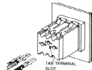
Quick connect mounting (5.2mm x 0.5mm)
