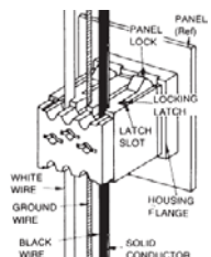
Solid Wire connection (12-14AWG)
