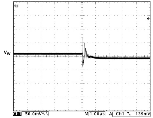
Figure 25. Midscale Glitch, Code 0x80 to Code 0x7F
