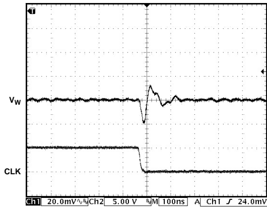
Figure 22. Digital Feedthrough
