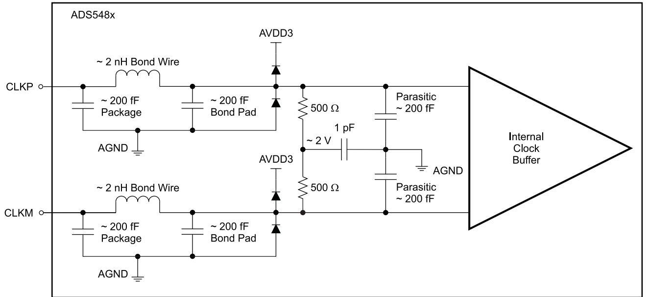
Figure 67. Clock Input Circuit
