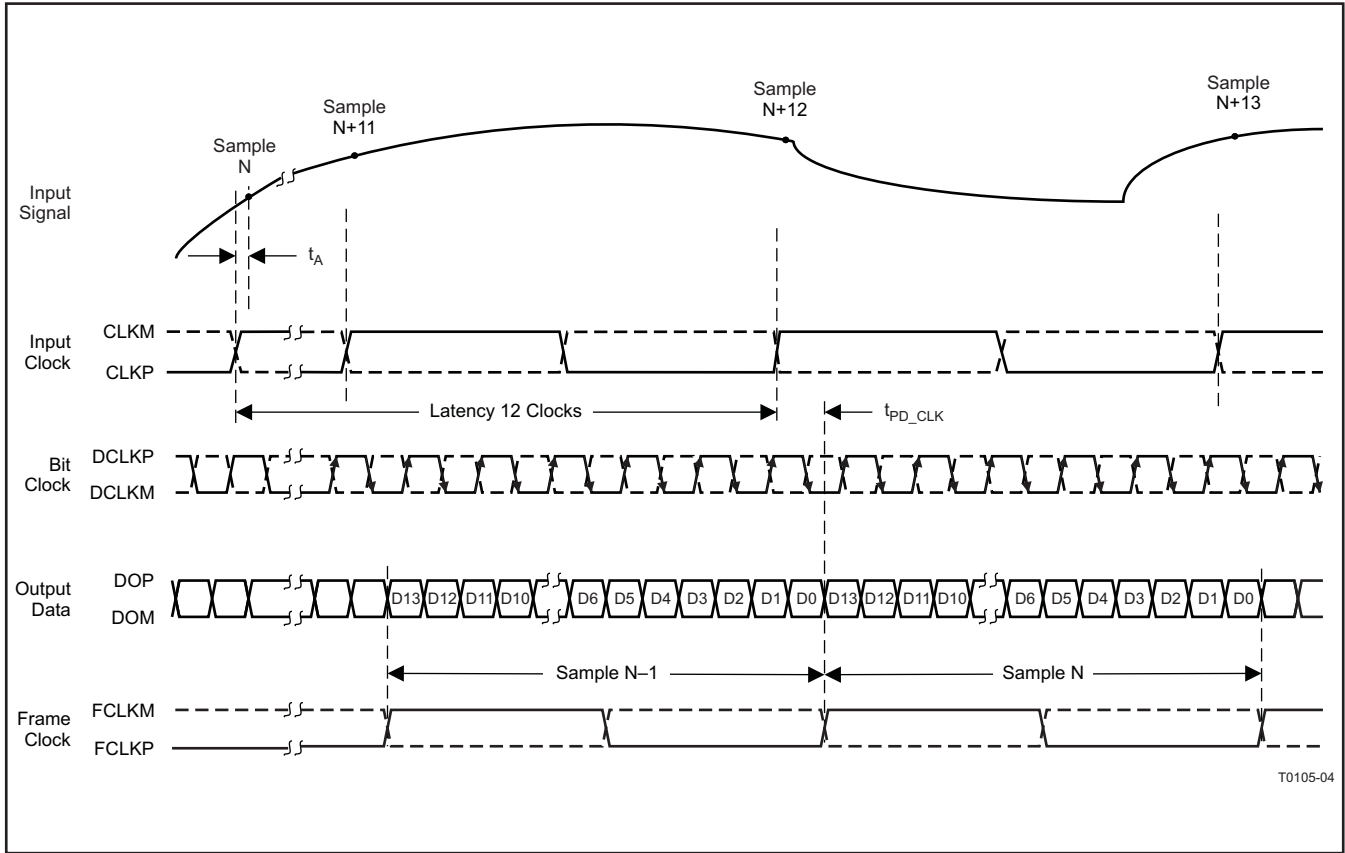
Figure 1. Latency
