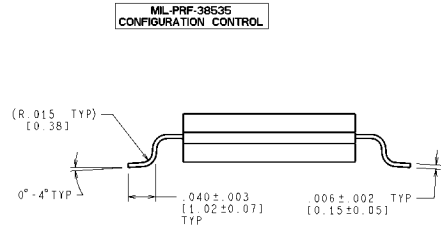
16 Lead Surface Mount Package (WG) See NS Package Number WG16A
