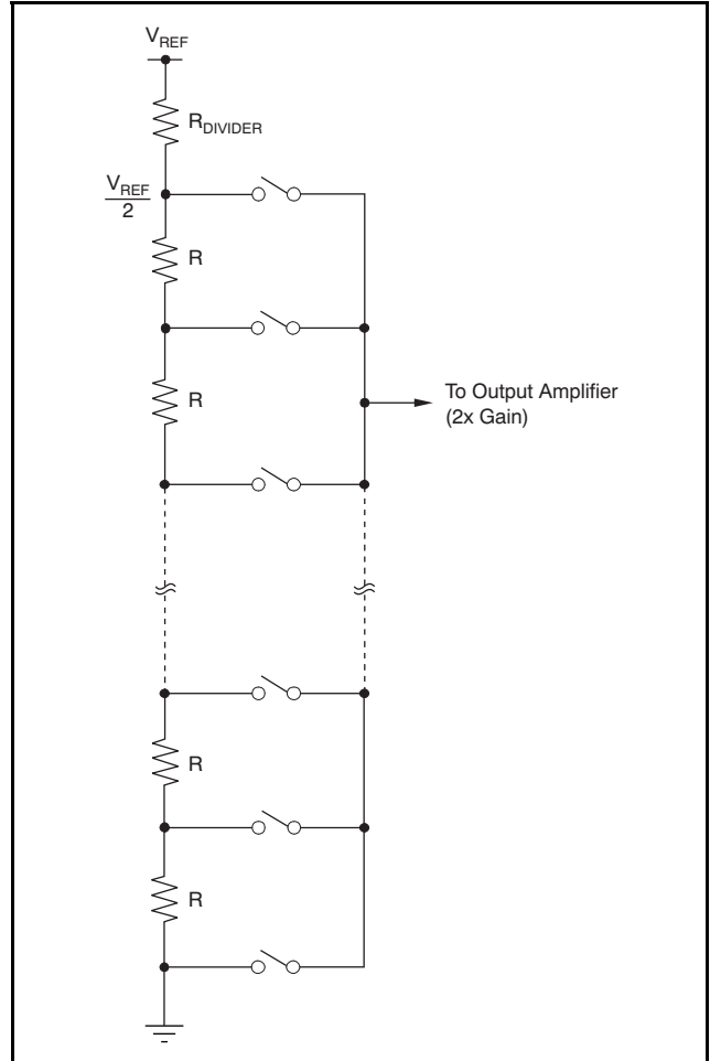
Figure 63. Resistor String
