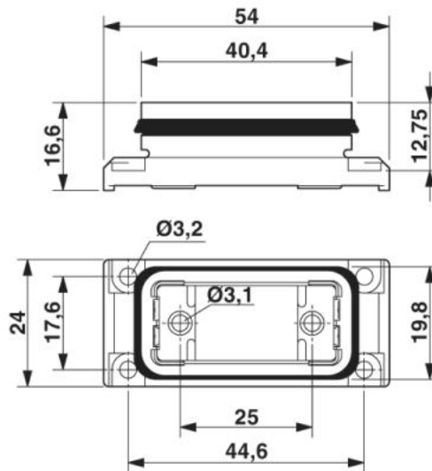
D-SUB panel mounting frame
