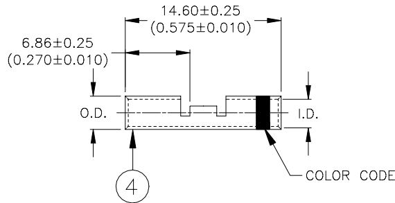
ITEM #2: CRIMP SPLICE
