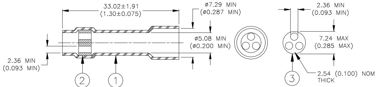
ITEM #1: SEALING SLEEVE
