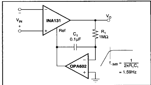
FIGURE 10. AC-Coupled Instrumentation Amplifier.
