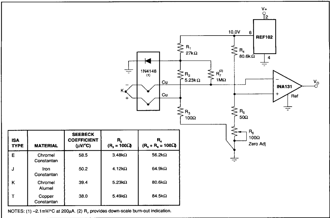
FIGURE 8. Thermocouple Amplifier with Cold Junction Compensation.
