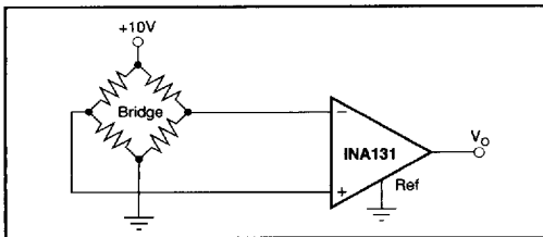
FIGURE 9. Bridge Transducer Amplifier.
