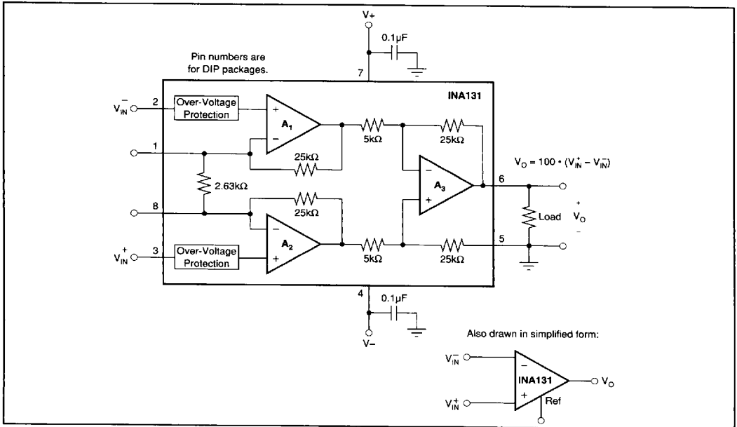
FIGURE 1. Basic Connections.
