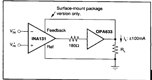
FIGURE 5. Buffered Output for Heavy Loads.
