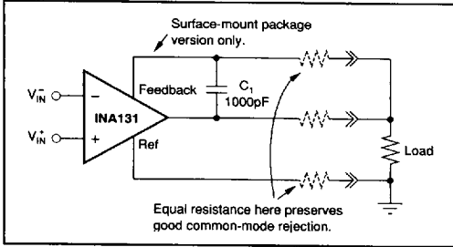
FIGURE 4. Remote Load and Ground Sensing.
