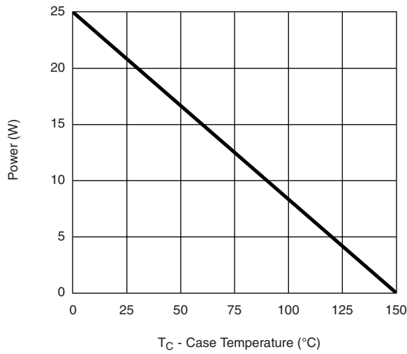
Power, Junction-to-Case
