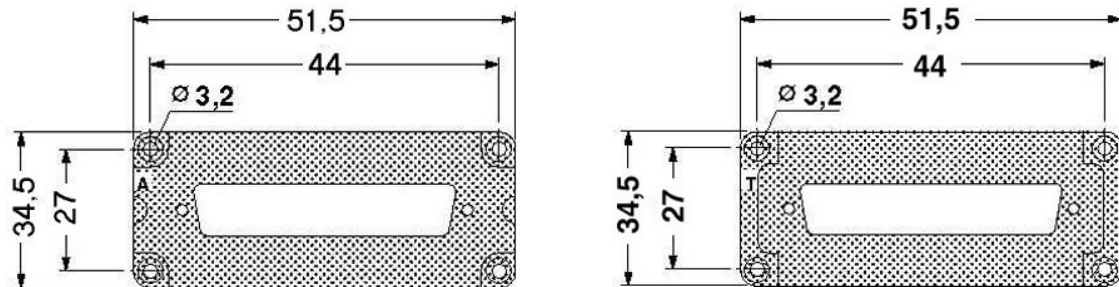
Dimensioned drawing
