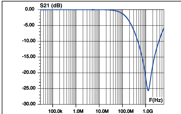
Figure 9. S21 attenuation measurement results of each channel
