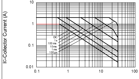
Safe Operating Area
