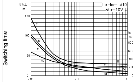
Switching Speeds
