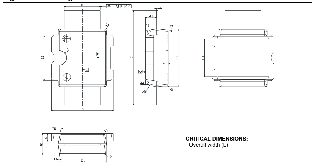
Figure 16. Package dimensions
