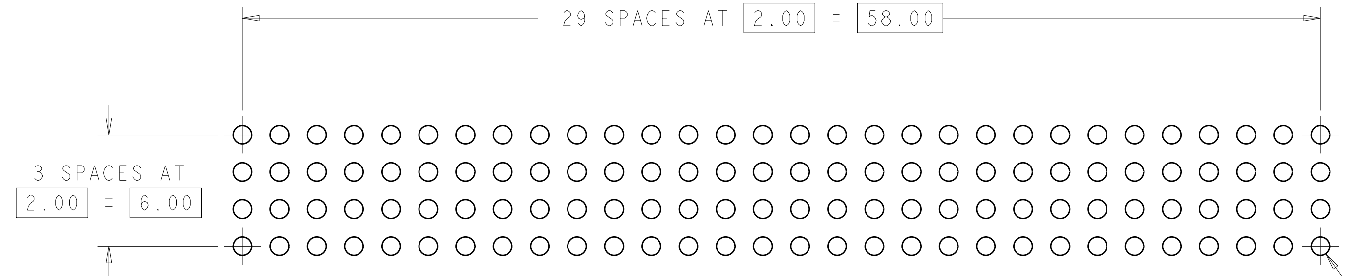
RECOMMENDED PCB LAYOUT FOR 1375967-1 & -4
