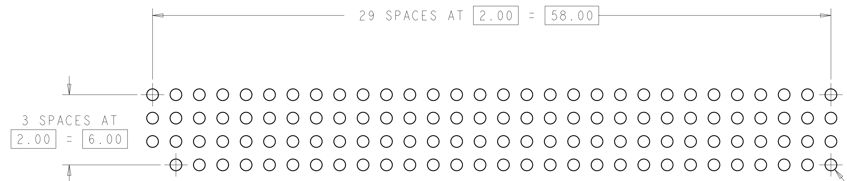
RECOMMENDED PCB LAYOUT FOR 1375967-2 & -5
