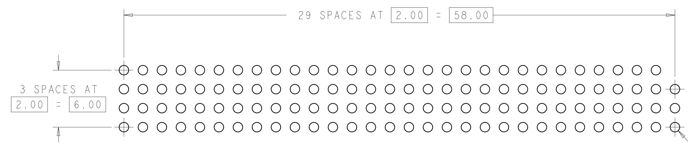
RECOMMENDED PCB LAYOUT FOR 1375967-3 & -6
