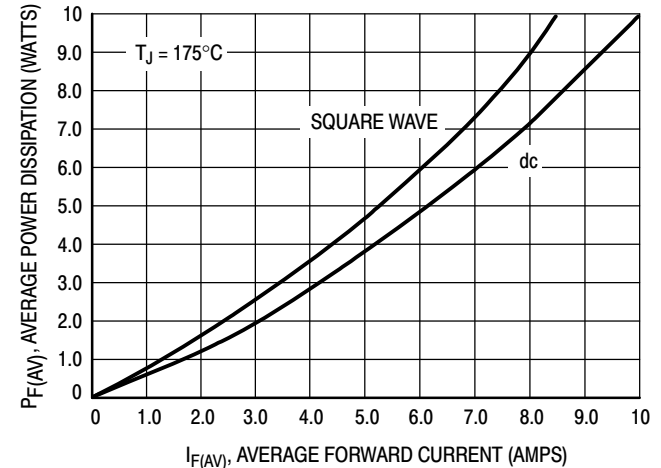
Figure 10. Power Dissipation
