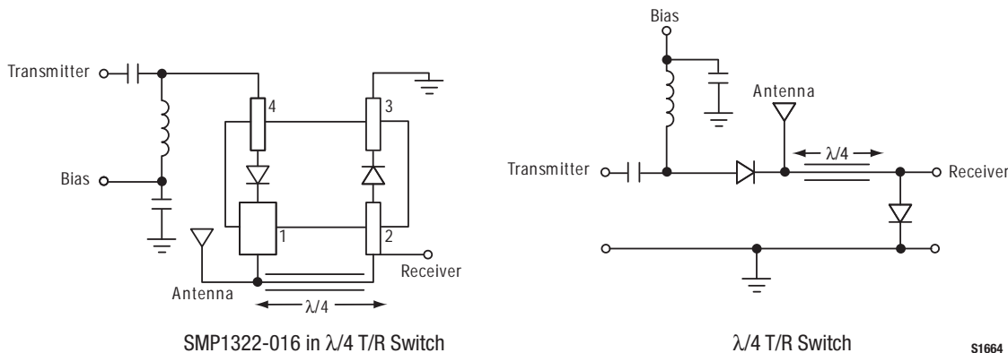
Figure 1. SMP1322-016 Quarter-Wave T/R Switch
