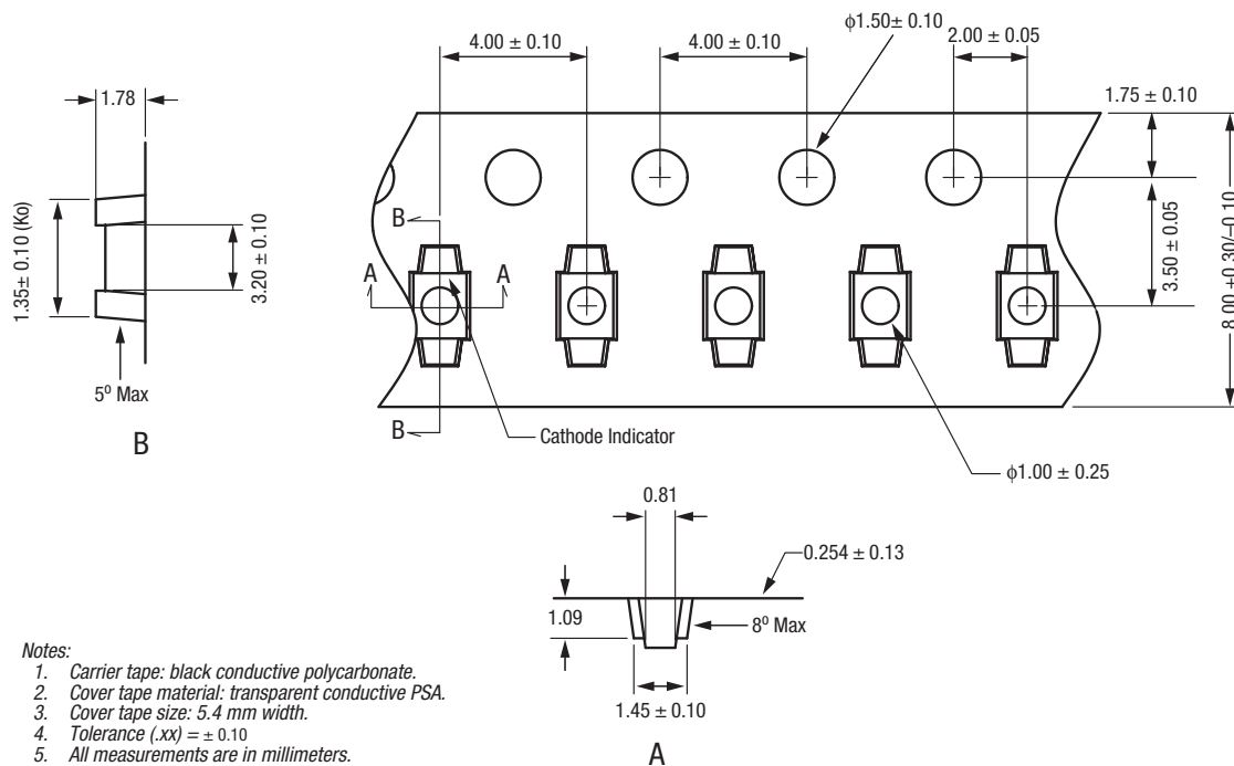
Figure 13. SOD-323 Tape and Reel Dimensions
